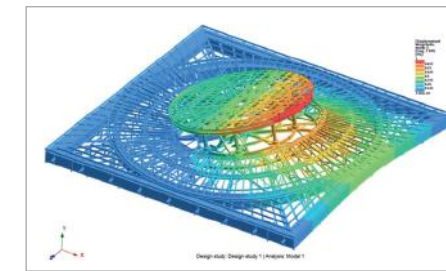
A complex assembly like this one, with 5200 parts, can be analyzed in minutes
