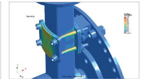
Nonlinear analysis accurately reproducing the contact between bolt and plate
