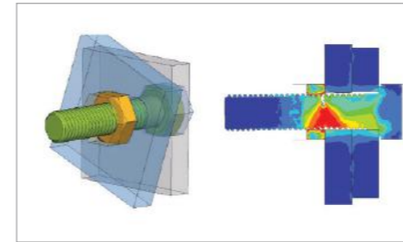
Bolt modeling with material failure
