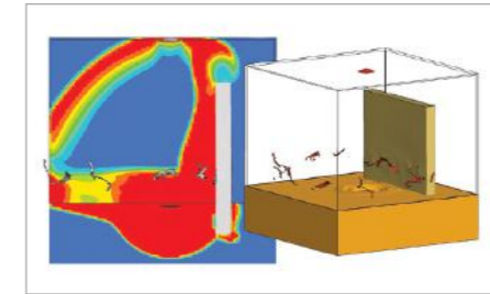
FSI application: Steel casing and concrete wall under explosion load (Fluid-structure Interaction)
